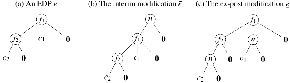
FIGURE 7: Interim and Ex-post Participation Constraints in Frame n
