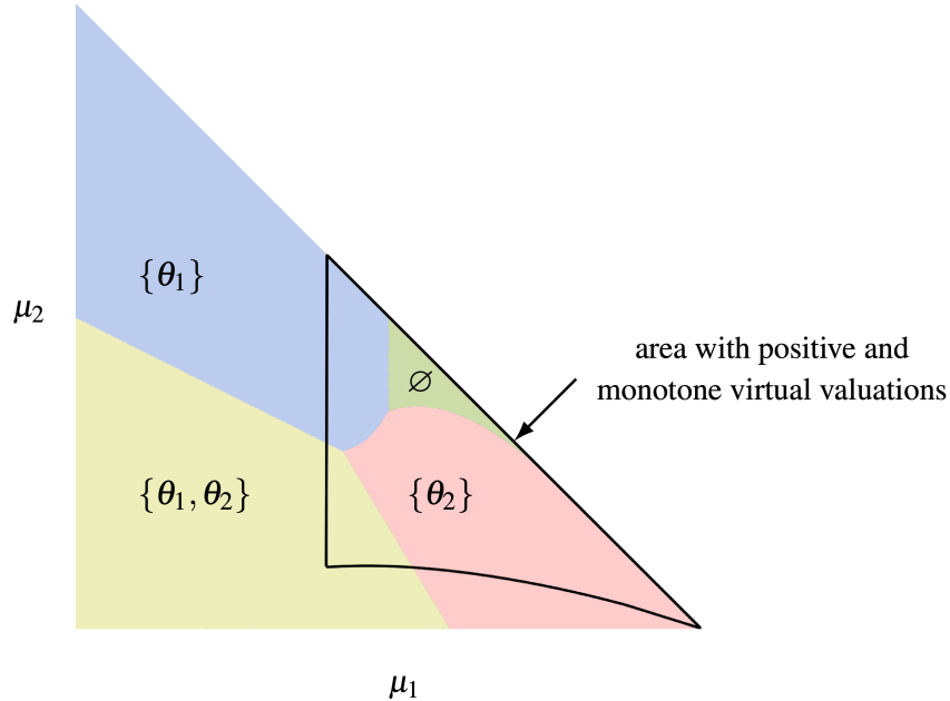
FIGURE 5: Optimal \Theta_C for \theta^1 = (1, 3) , \theta^2 = (4, 5) , \theta^3 = (5, 6) .
