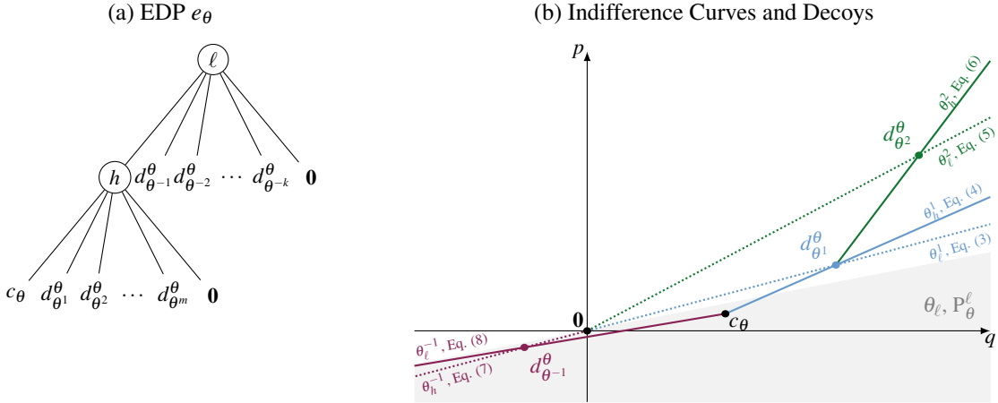
FIGURE 3: The construction of e_\theta .
