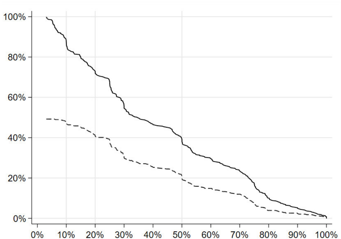
Figure 2: Reverse cumulative distribution of the largest shareholding in a sample of 384 listed German stock corporations as of December 2017. 51 The straight line shows the percentage of companies (vertical axis) with a largest shareholder directly or indirectly holding at least as many voting rights as shown on the horizontal axis. The dashed line represents the corresponding percentage of natural persons as largest shareholders.
